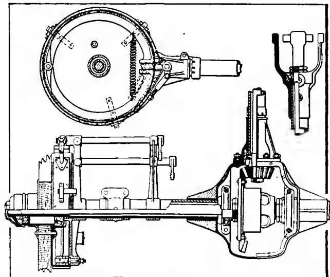
Fig. 11—Transverse section through National rear axle assembly, showing details of brake construction and differential
